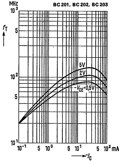
Transition frequency f_T = f(I_C) T_{amb} = 25^\circ\text{C}; V_{CE} = \text{parameter}
