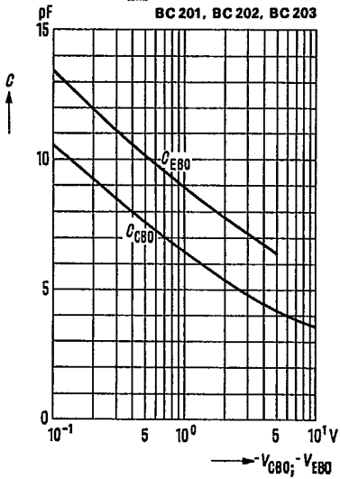
Collector-base capacitance C_{CBO} = f(V_{CBO}) Emitter-base capacitance C_{EBO} = f(V_{EBO}) f = 1\text{ MHz}; T_{amb} = 25^\circ\text{C}
